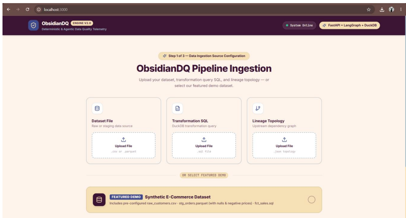
Figure 7.2: Screen 1 Dataset Upload and Preset Selection (UploadStep.tsx)
