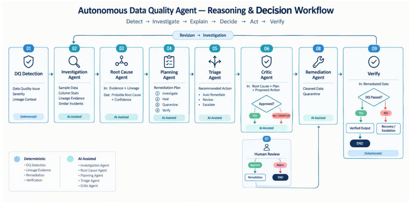
Figure 4.3: Agentic Investigation, Planning and Triage
