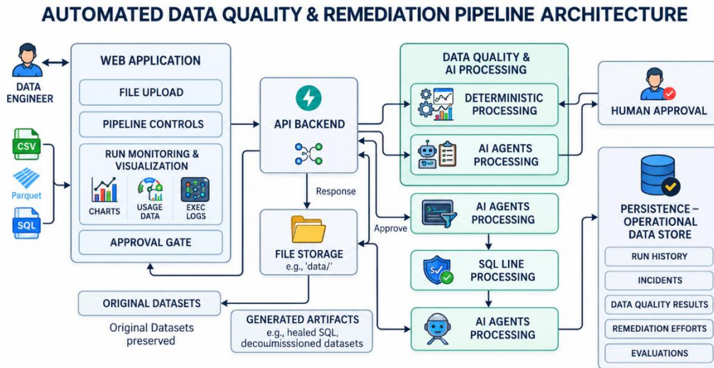
Figure 3.1: Overall ObsidianDQ System Architecture
